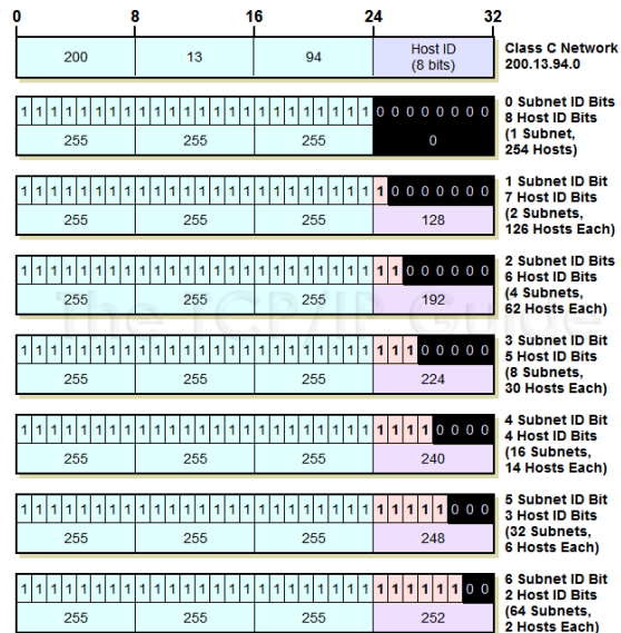
Figure 69: Custom Subnet Masks for Class C Networks
