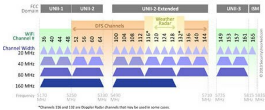
802.11ac Channel Allocation (N America)
