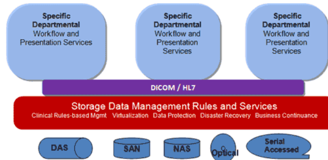
Figure 7-2: Storage Data Management Rules and Service
