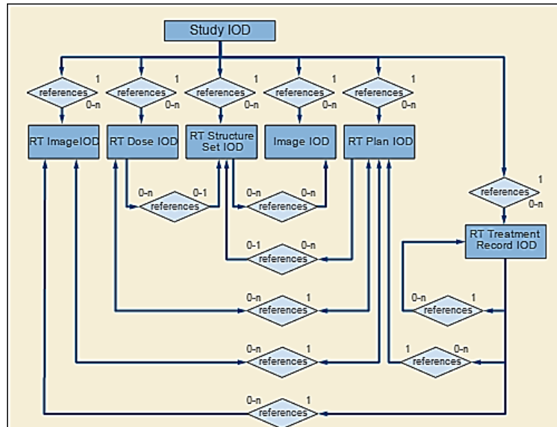
Figure 7-2c. DICOM Information Model - RADIOTHERAPY
